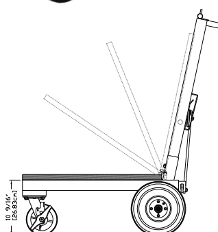
Cable X-Over Cart shown with optional (Aluminum) Folding Plate
