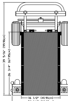
E-13 Shown with optional Folding Plate up
