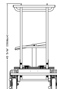
Cable X-Over Cart shown with optional (Aluminum) Folding Plate
