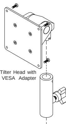
Mag LCD 4" Tilt Head Pin Adapter
