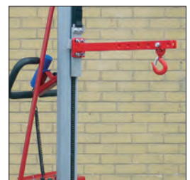
Jib and Hook - EP07 500mm long Capacity: 150kg £195.00
