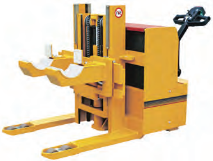
Axle Lifter
