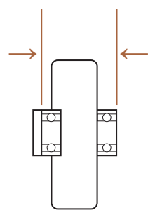
MOUNTING WIDTH
