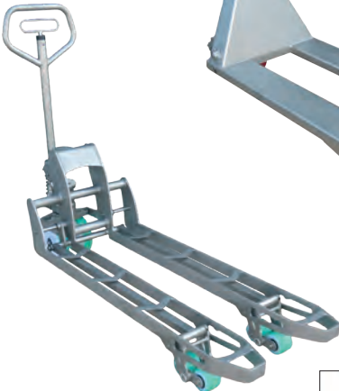
P20S-520x1150
